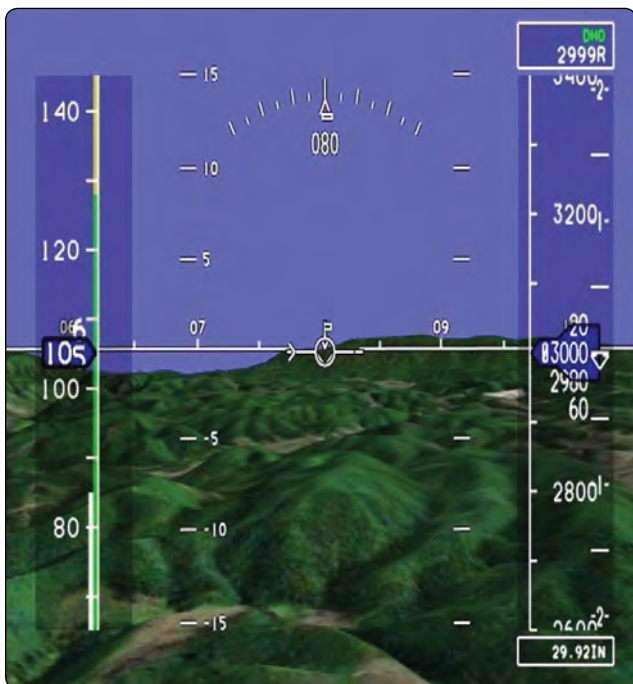
Figure 17-24. SVS system.
