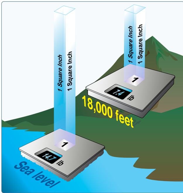
Figure 12-4. Atmosphere weights.
