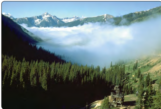
Figure 12-21. Radiation fog.
