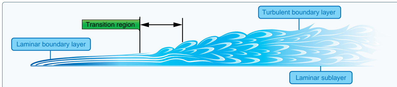
Figure 5-66. Boundary layer.
