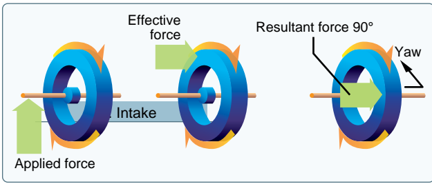
Figure 5-49. Gyroscopic precession.
