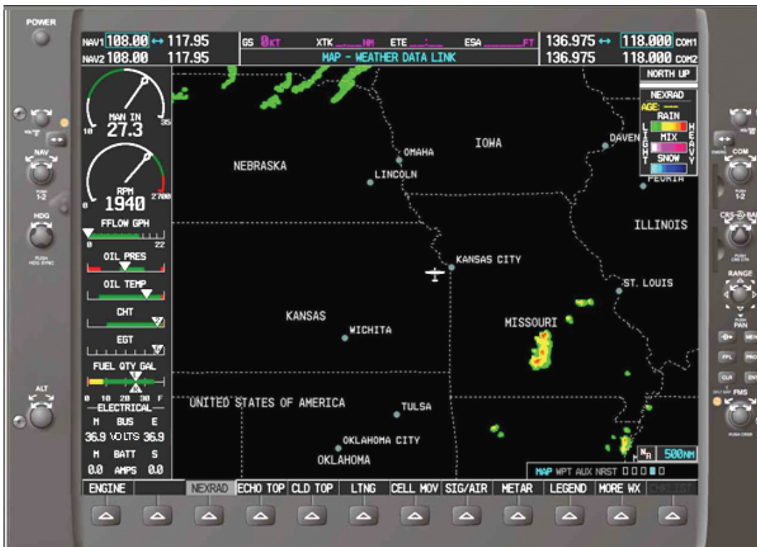
Figure 13-18. NEXRAD radar display (500 mile range). The individual color gradients can be easily discerned and interpreted via the legend in the upper right corner of the screen. Additional information can be gained by pressing the LEGEND soft key, which displays the legend page.
