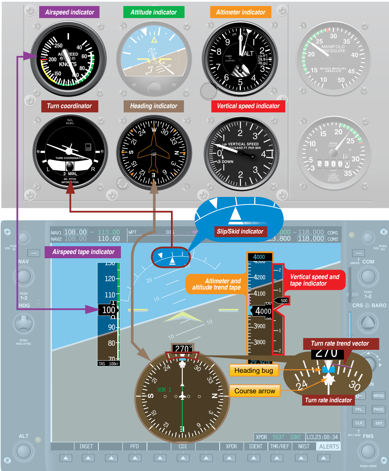
Figure 3-19. Performance instruments.
