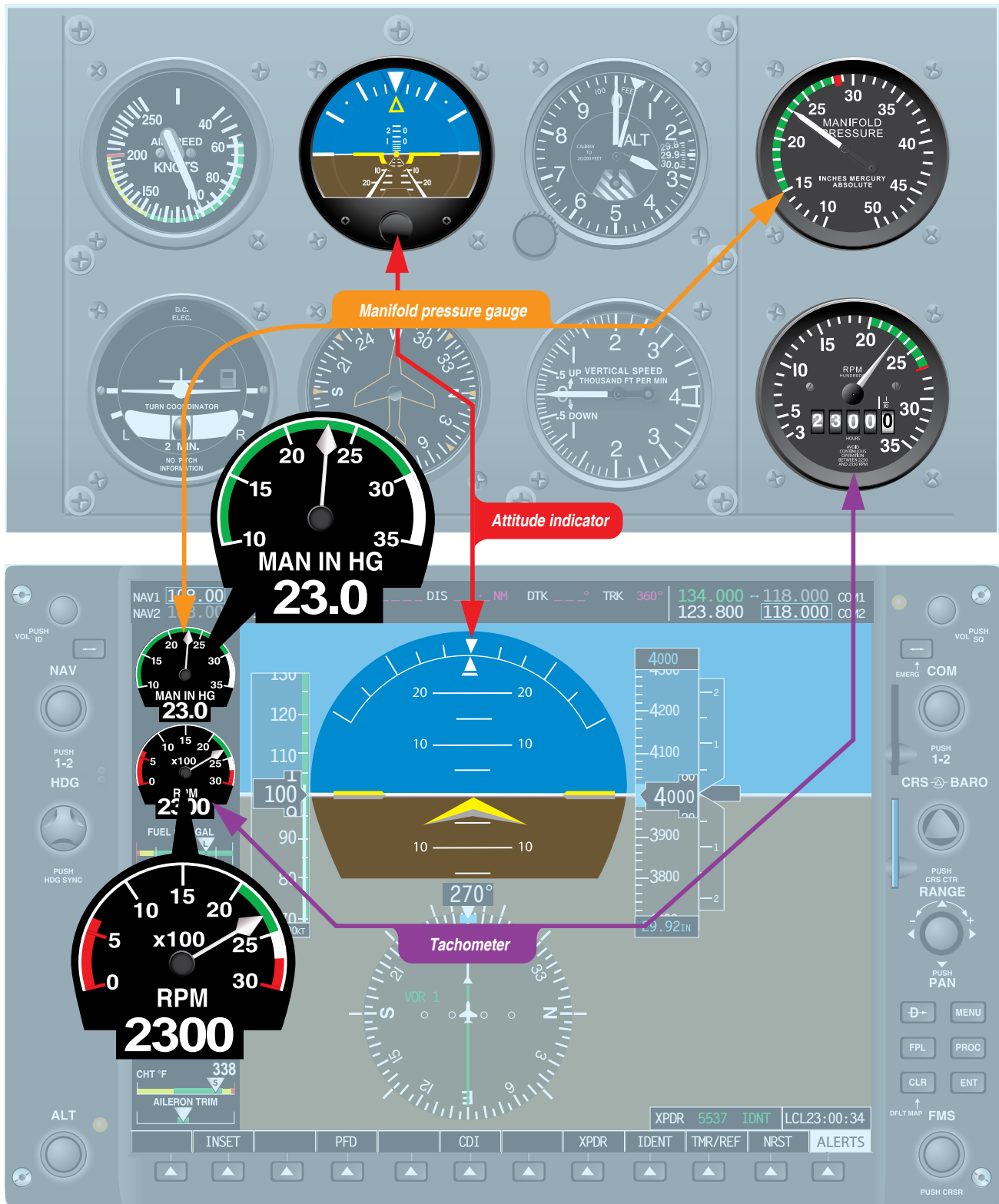
Figure 3-20. Control instruments.
