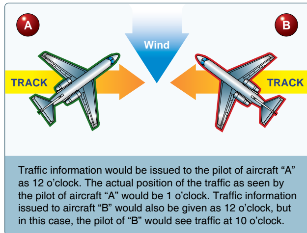
Figure 14-44. Traffic advisories.
