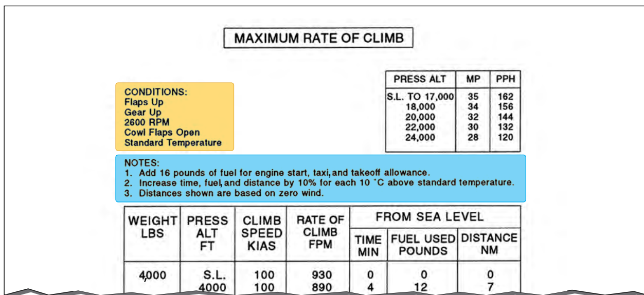
Figure 11-20. Conditions notes chart.
