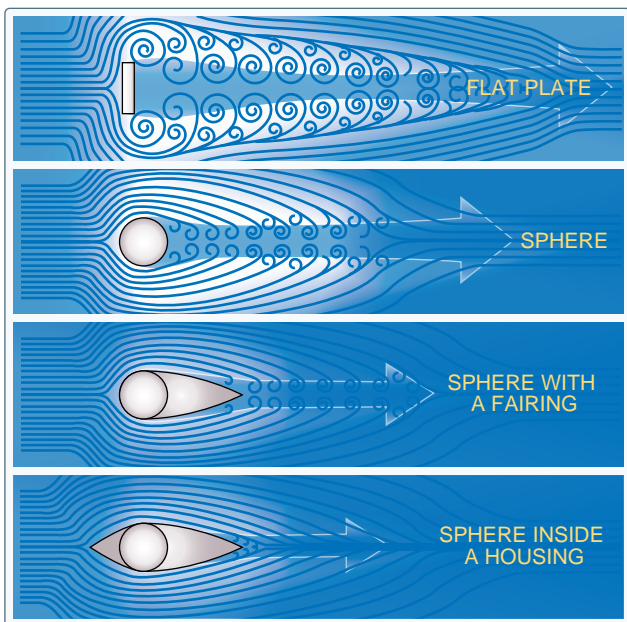
Figure 5-7. Form drag.
