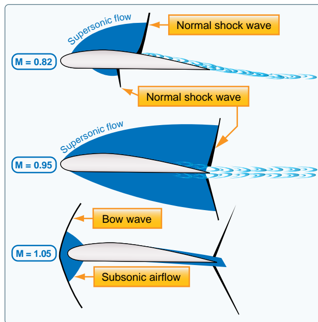
Figure 5-67. Shock waves.
