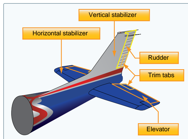
Figure 3-10. Empennage components.
