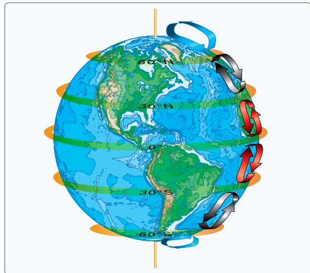
Figure 12-5. Three-cell circulation pattern due to the rotation of the Earth.
