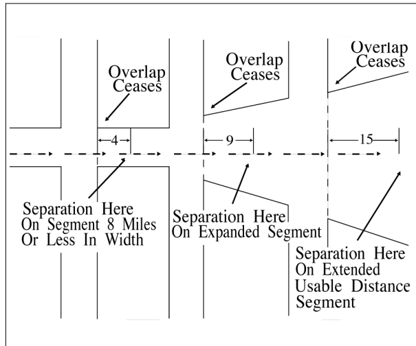
FIG 6–5–8 RNAV Minima
